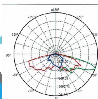
Distribution Curve [Unit:cd]
