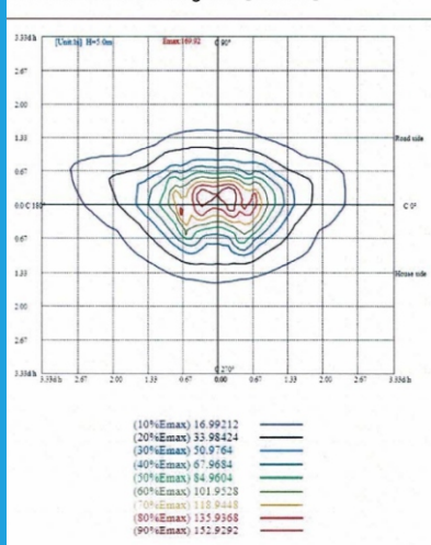
ISO illuminance diagram [Unit:lx]
