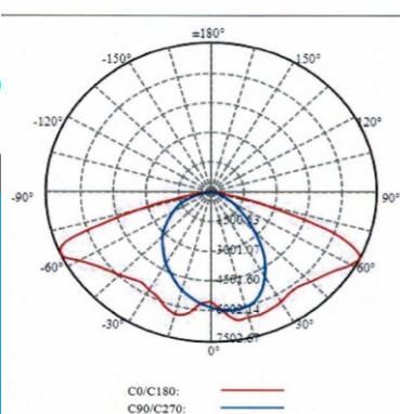
Distribution Curve [Unit:cd]
