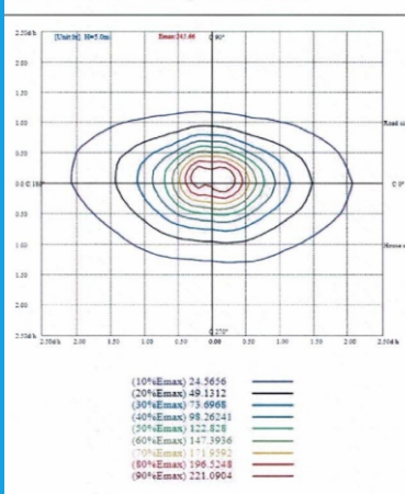
ISO illuminance diagram [Unit:lx]
