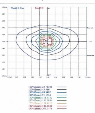
ISO illuminance diagram [Unit:lx]
