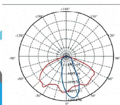
Distribution Curve [Unit:cd]
