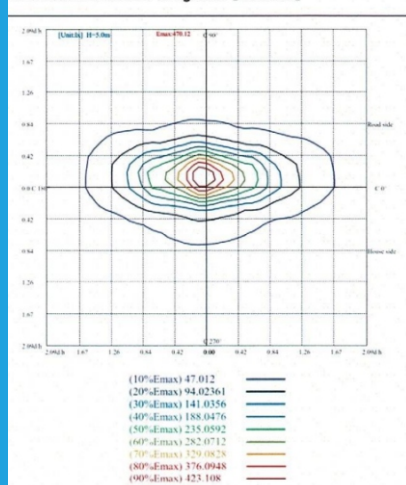
ISO illuminance diagram [Unit:lx]
