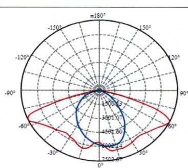
Distribution Curve [Unit:cd]
